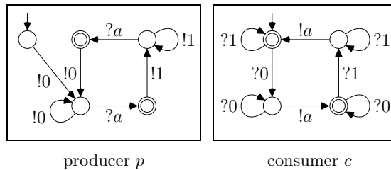
Fig. 2. Example CFM
