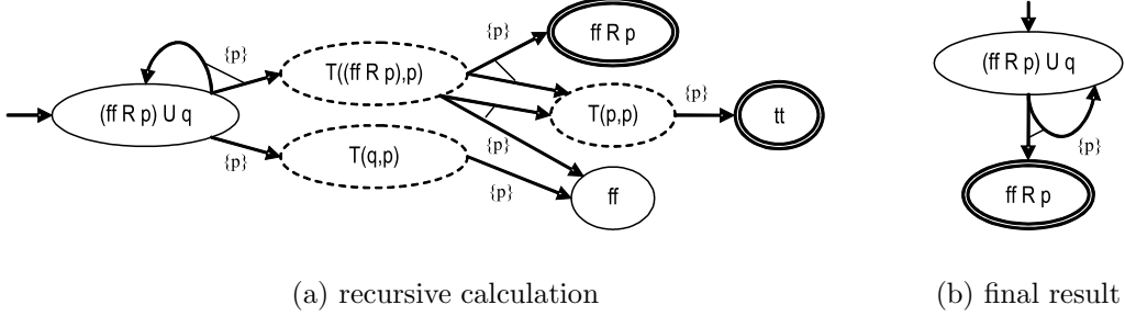
Fig. 1. Calculation of T(((\mathbf{ff} \mathbf{R} p) \mathbf{U} q), \{p\})
